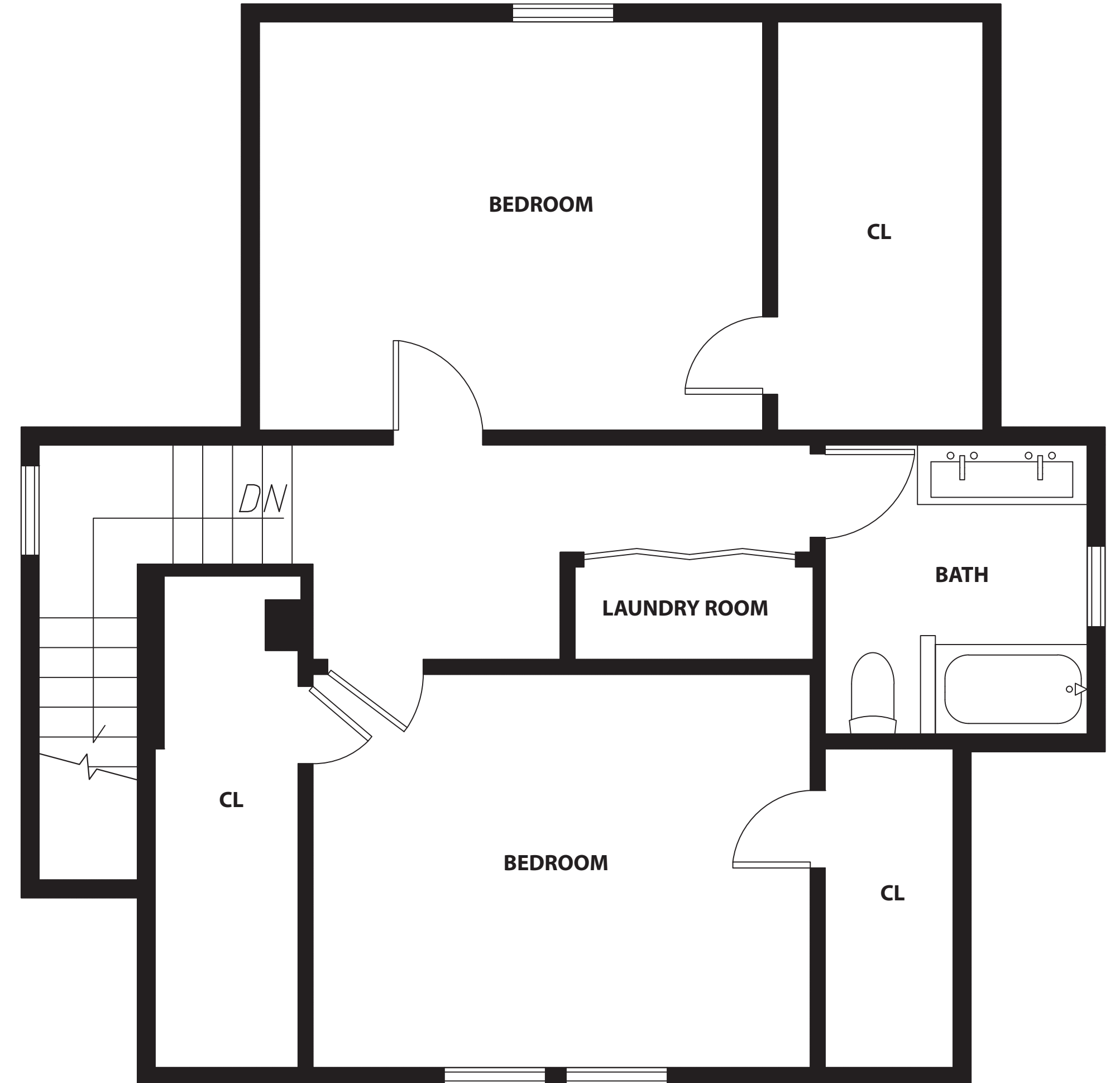
THIRD FLOOR
