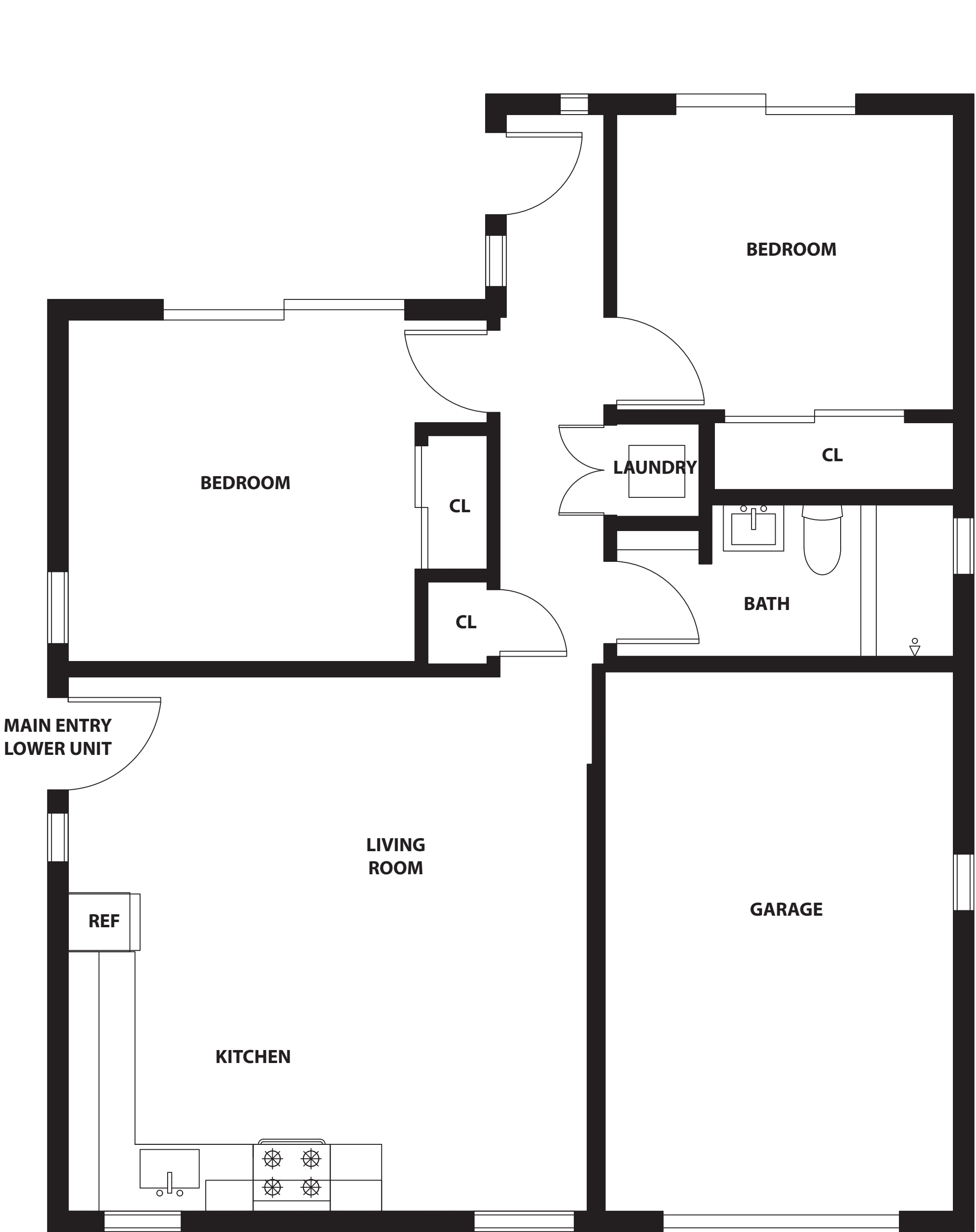
FIRST FLOOR
